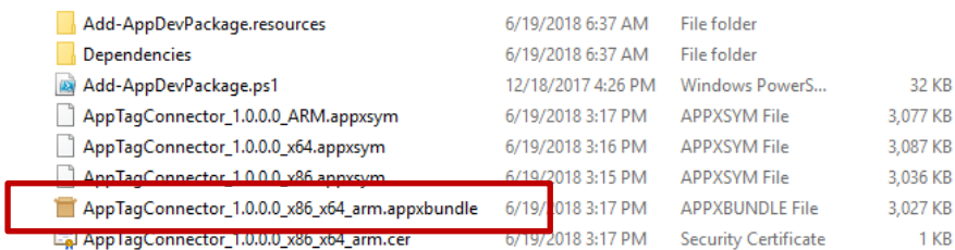
Figure 26 - Install package
