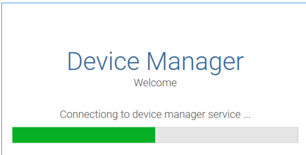
Figure 28 – Home screen
