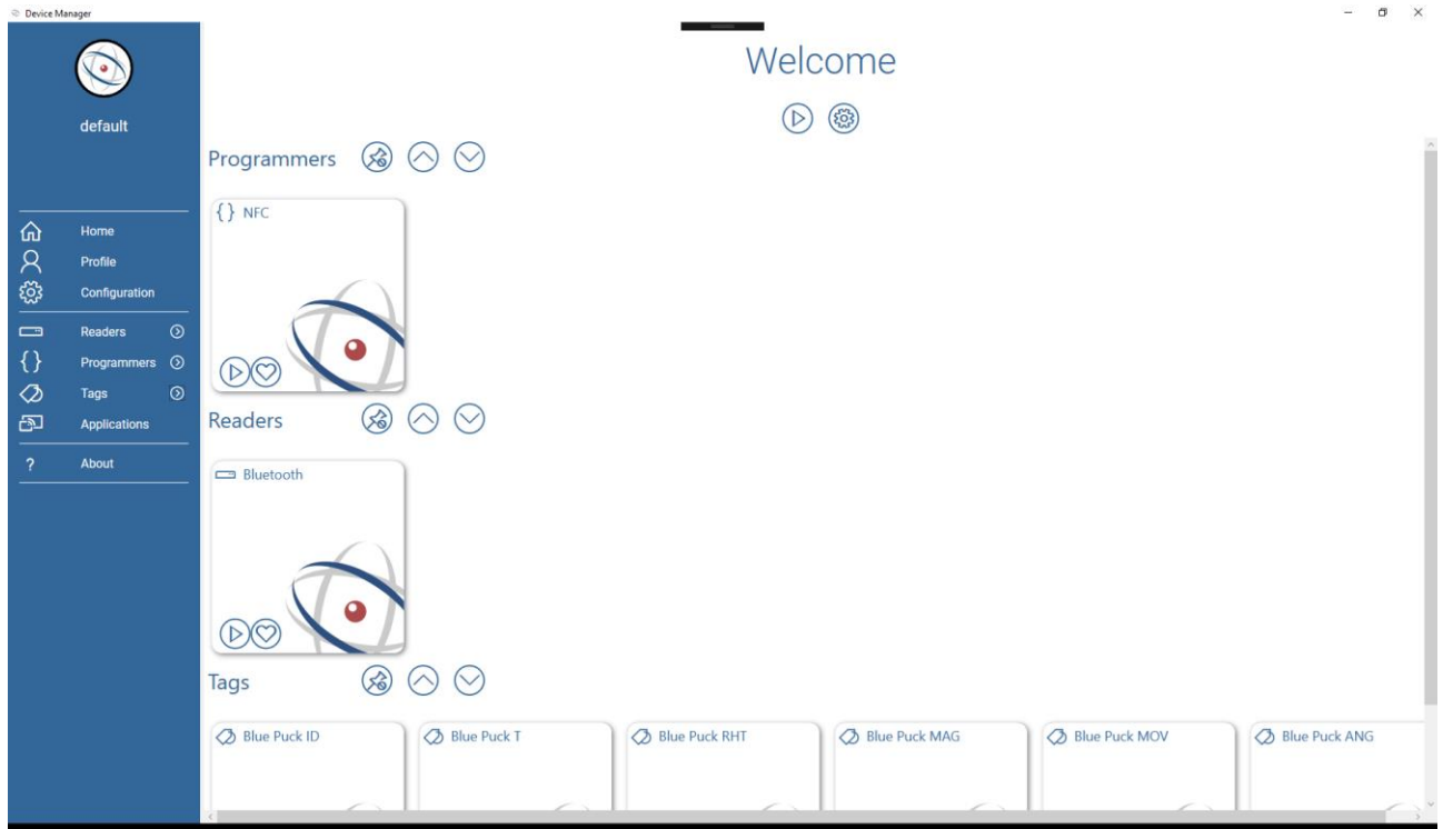
Figure 35 - Dashboard
