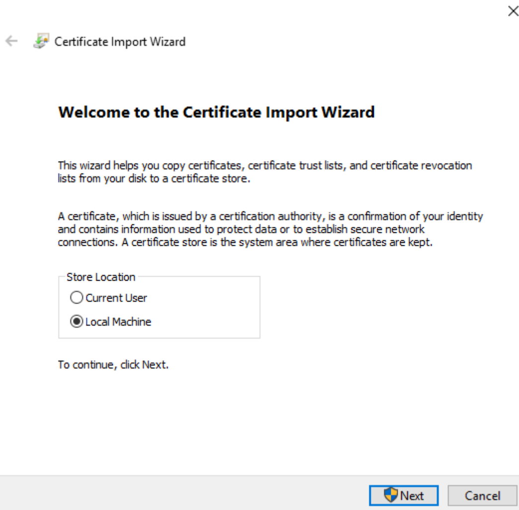
Figure 19 – First step
