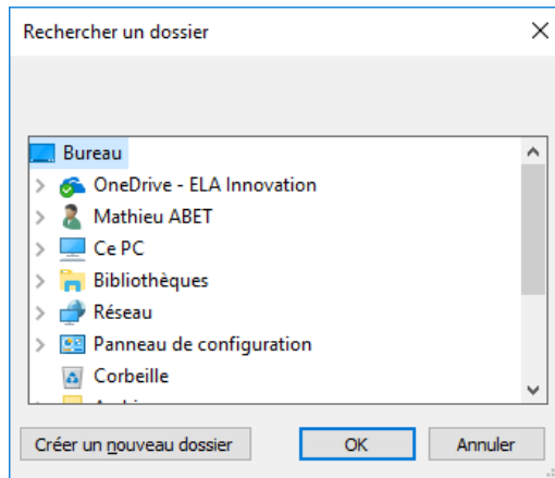
Figure 49 – Environment back-up
