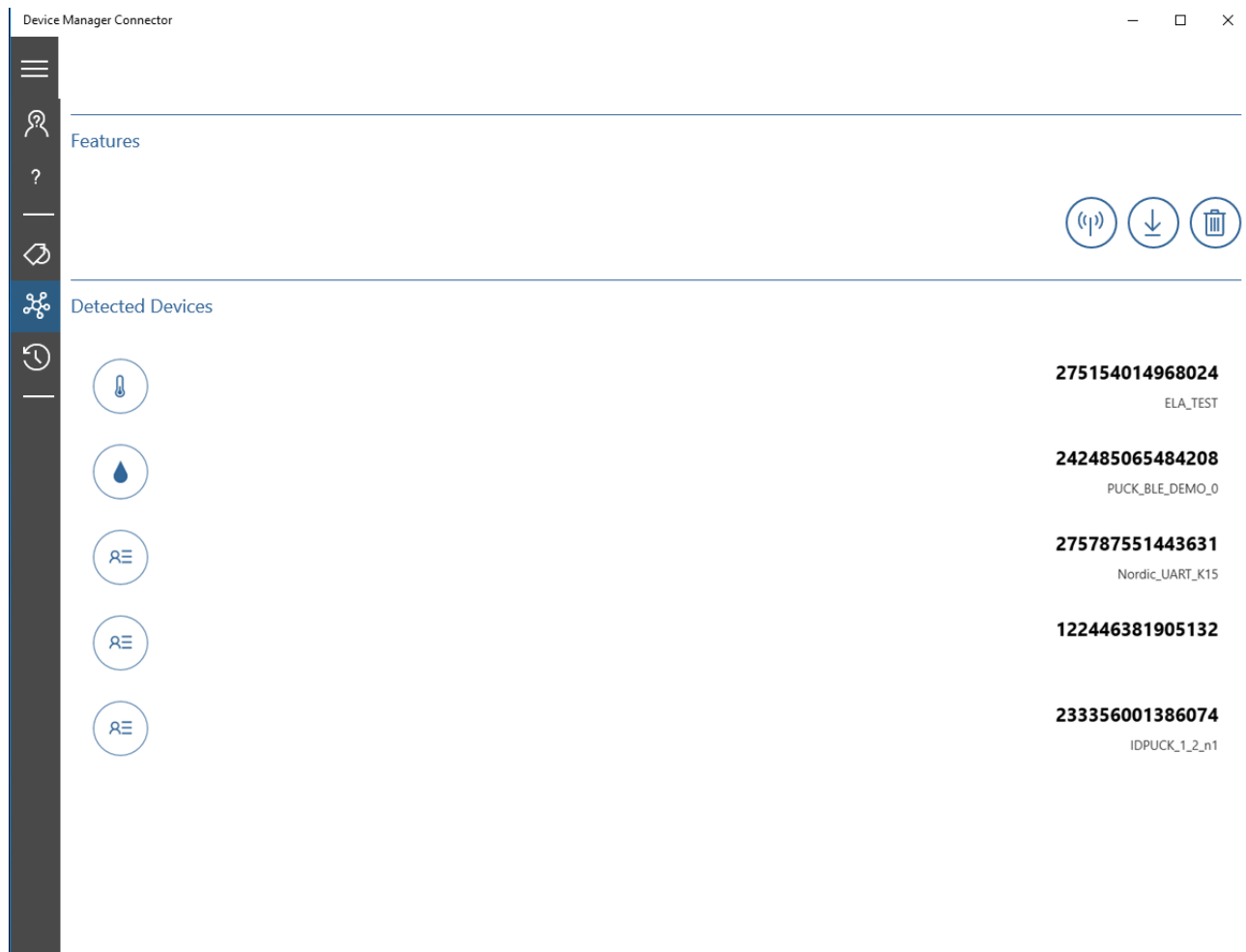
Figure 143 - scan IoT
