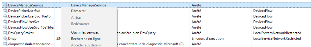
Figure 156 – Service management
