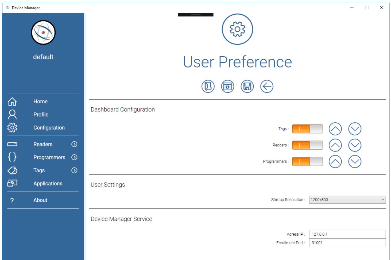
Figure 46 - Control panel
