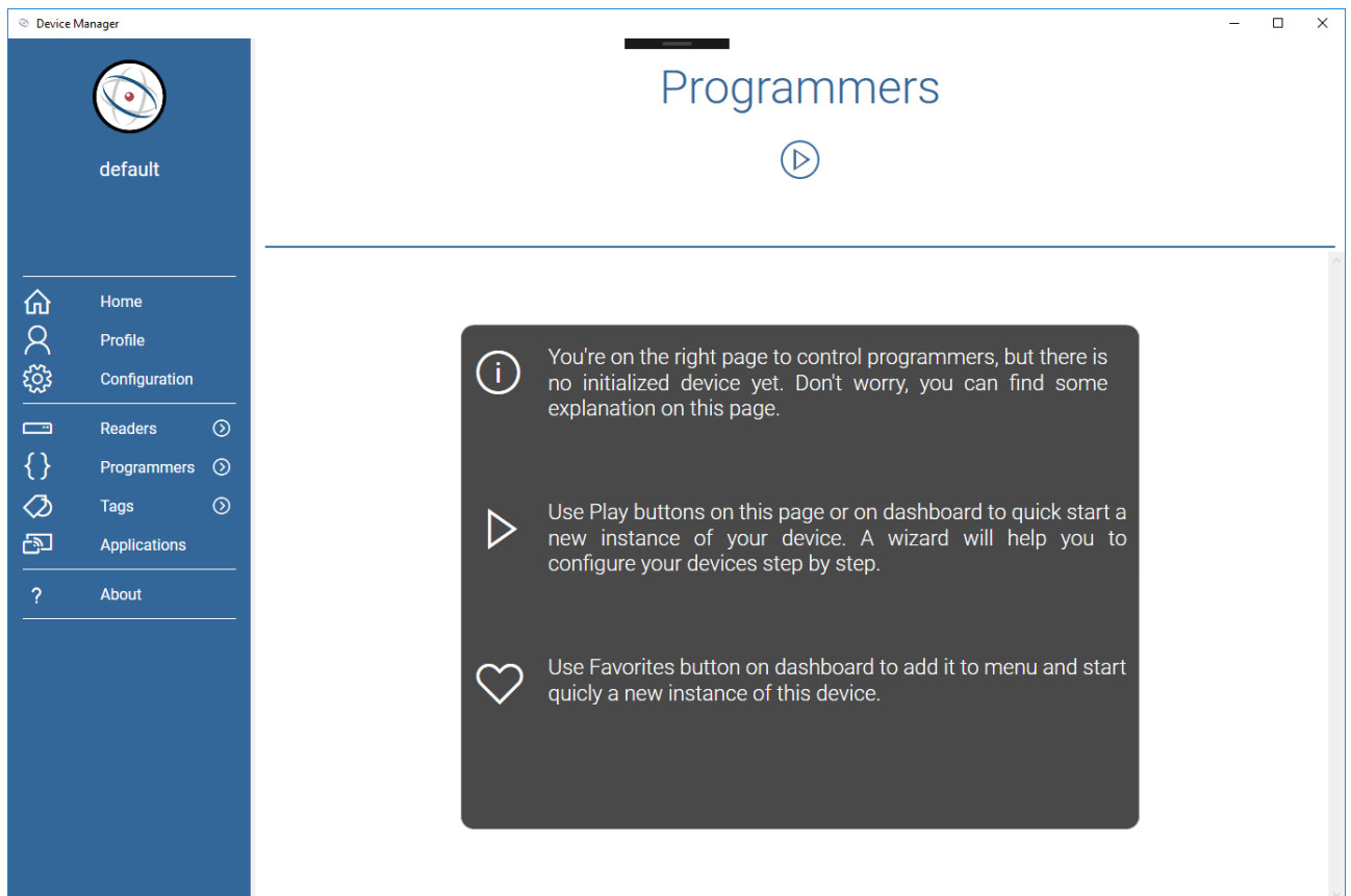
Figure 61 - Programmers panel
