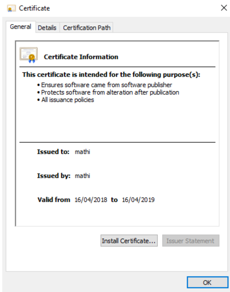
Figure 18 – Certificate window
