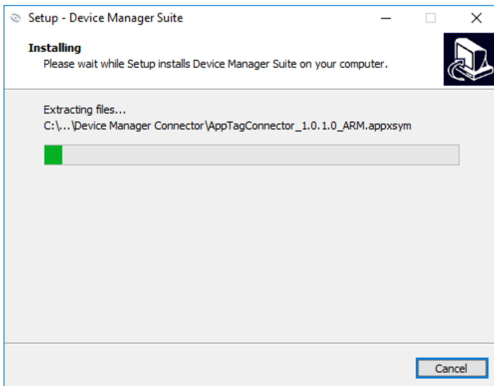
Figure 8 – Installation progress
