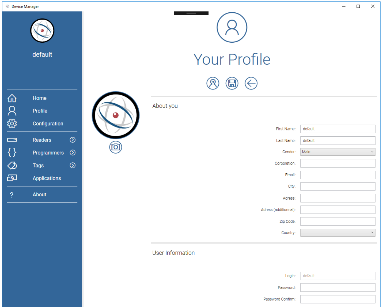
Figure 42 – User profile
