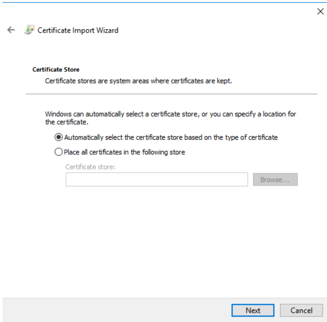
Figure 20 – Second step
