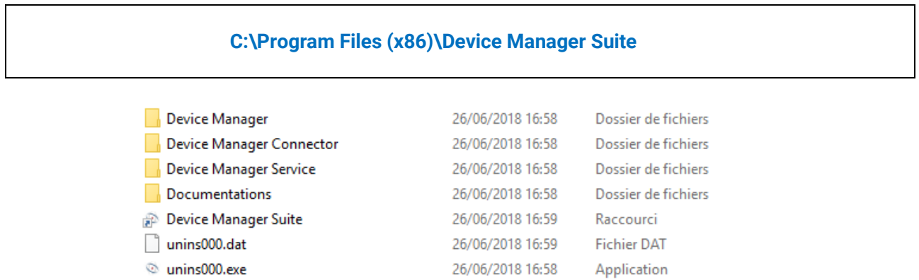
Figure 157 – Installation directory
