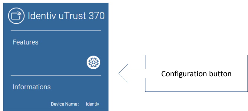
Figure 64 – NFC controller
