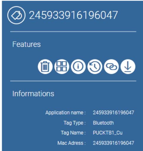
Figure 60 – Tags controller
