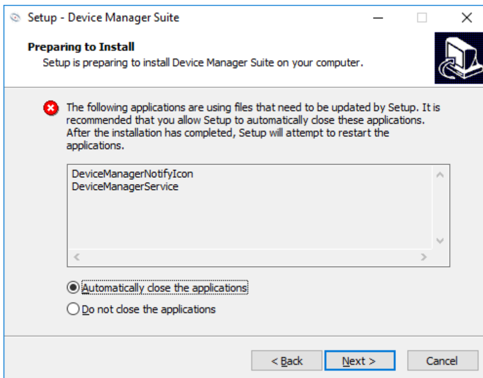
Figure 10 –Applications update
